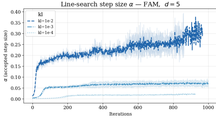
Figure 4: Accepted line-search step size \alpha over training for FAM at d = 5 (Adjoint Sampling), averaged over 5 seeds (shaded region: \pm 1 std). \alpha remains strictly positive and grows monotonically across all KL budgets \kappa , confirming that the line search does not degenerate under mini-batch gradients. Larger \kappa permits larger accepted steps.
