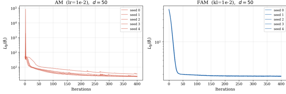
Figure 3: Loss curves for Adjoint Sampling. Left: Adam-only AM exhibits unstable, non-monotonic training. Right: FAM achieves a monotonic decrease in loss.
